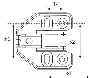
Adjustable mounting plate
